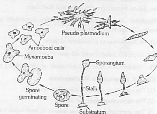
Fig : 1.3-4 Diagrammatic life cycle of cellular slime mould
